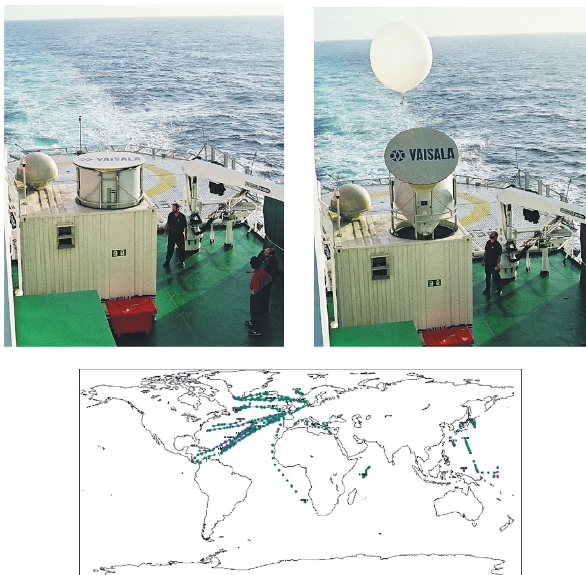
0344-F0011 Figure 11 The ASAP system is housed in either a standard 3 m (shown above) or 6 m sea container with a specially designed hatch to enable routine radiosonde launches in sustained winds up to 25 \text{ m s}^{-1} (gusts up to 35 \text{ m s}^{-1} ). (Bottom part) Worldwide ASAP radio soundings for November 2001.
