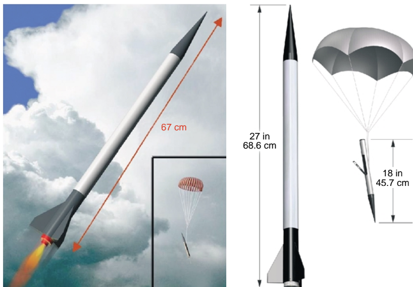
0344-F0012 Figure 12 Low-altitude rocketsonde unit with detached sonde descending on parachute (insert).
