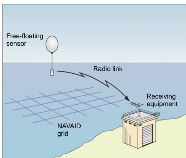
0344-F0006 Figure 6 NAVAID retransmission system.
