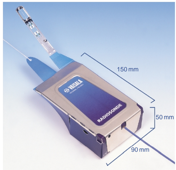
Figure 4 Vaisala RS90 Radiosonde with sensor boom.
