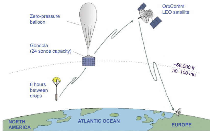
0344-F0010 Figure 10 The driftsonde system concept.
