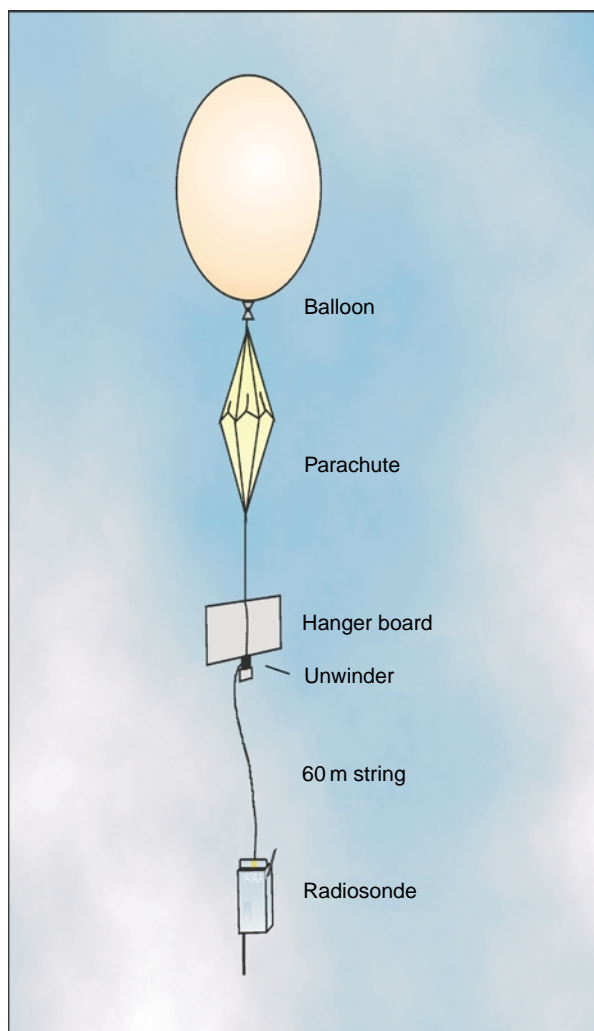
Figure 2 Typical radiosonde flight train, including balloon, parachute and hanger board, unwinder mechanism, separation line, and radiosonde. 0344-F0002
