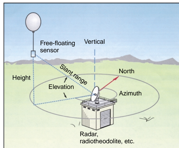
Figure 5 Angle-dependent tracking system.
